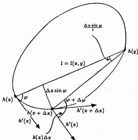
FIGURE 2. We can easily verify that the following formulas hold:
